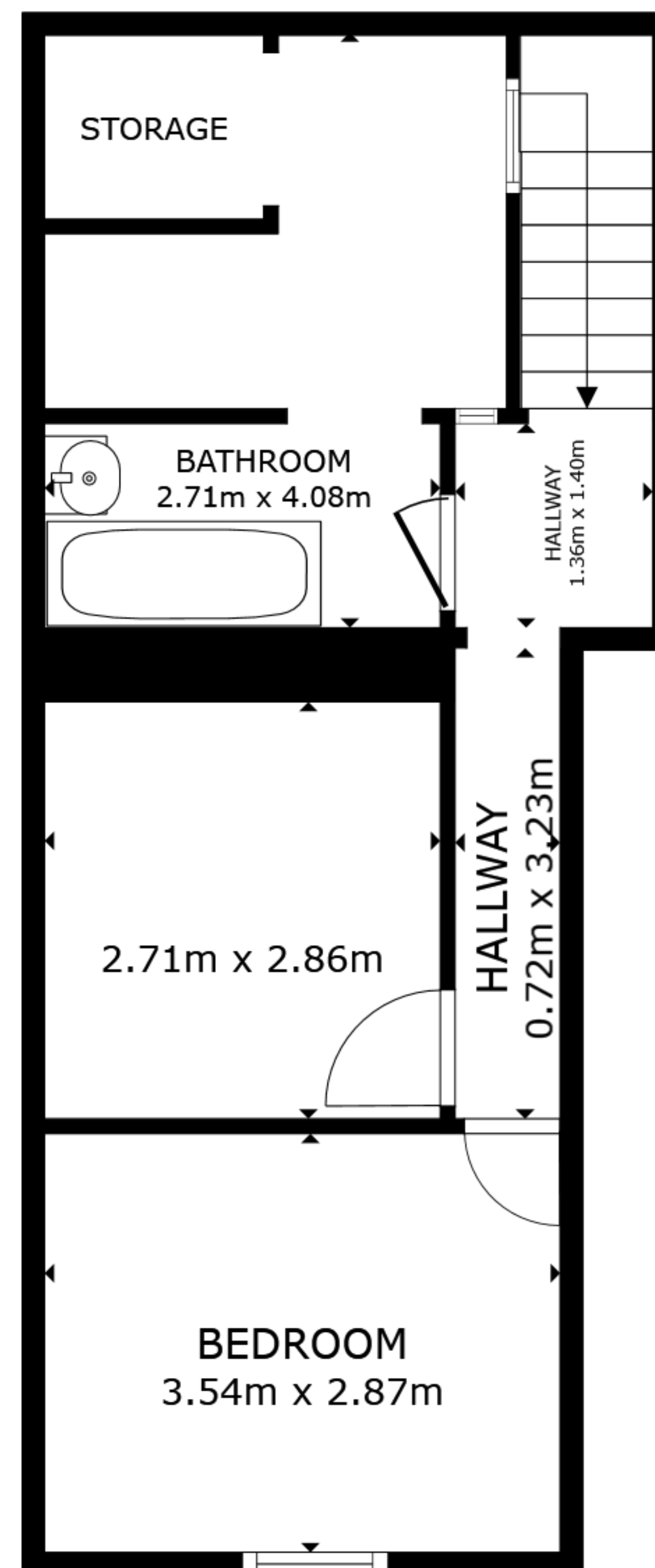
FLOOR 2
