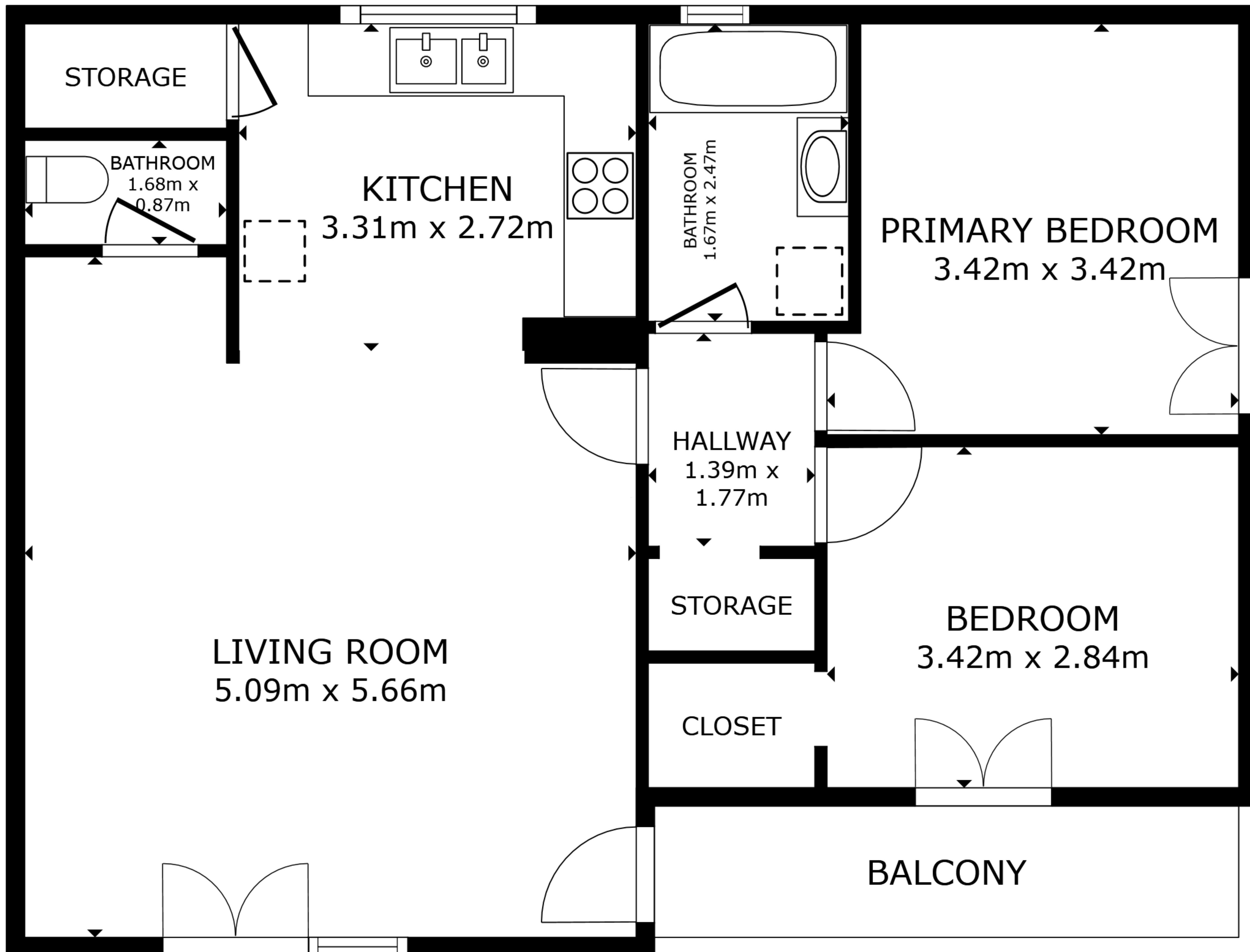
FLOOR PLAN
