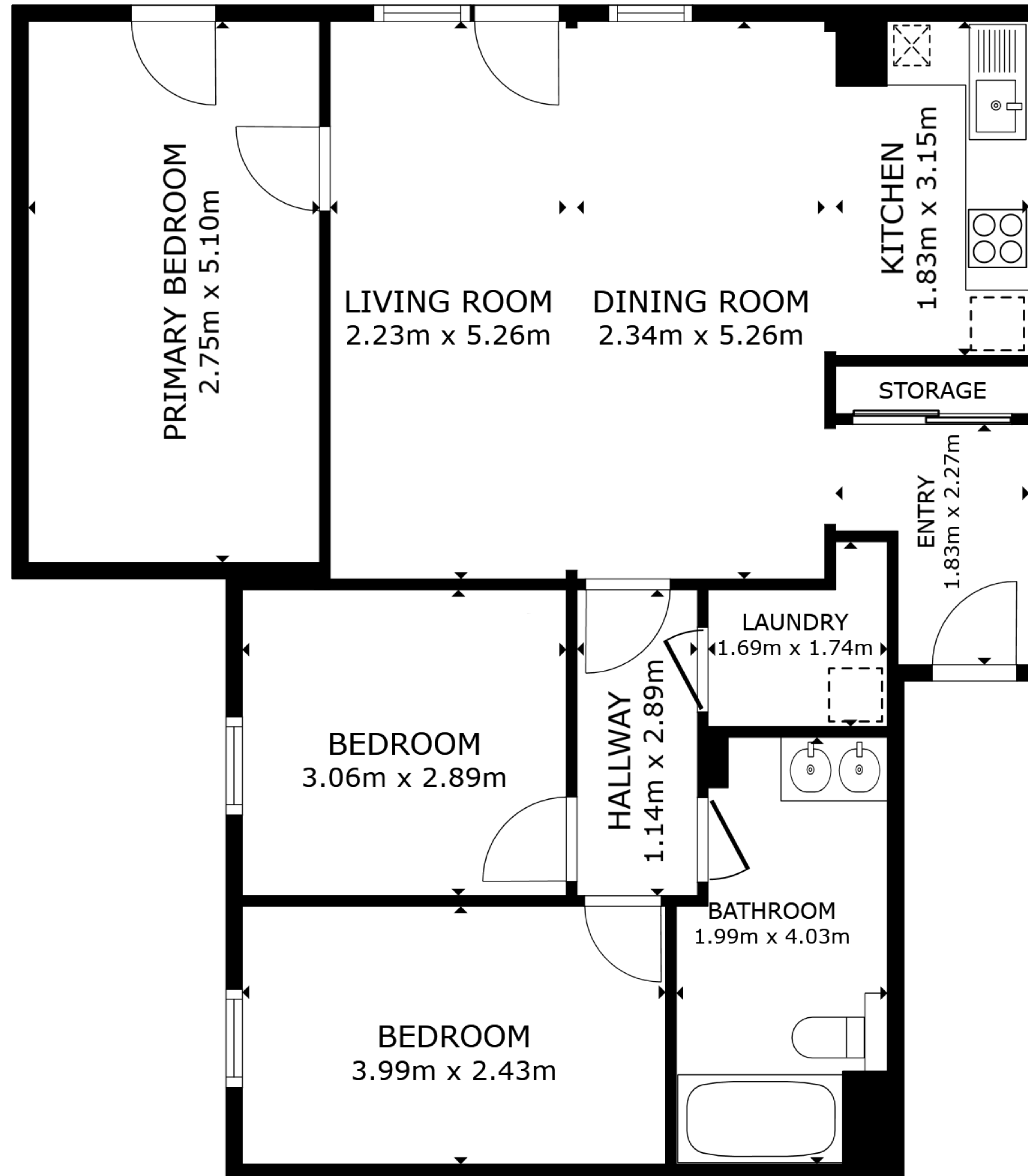
FLOOR PLAN
