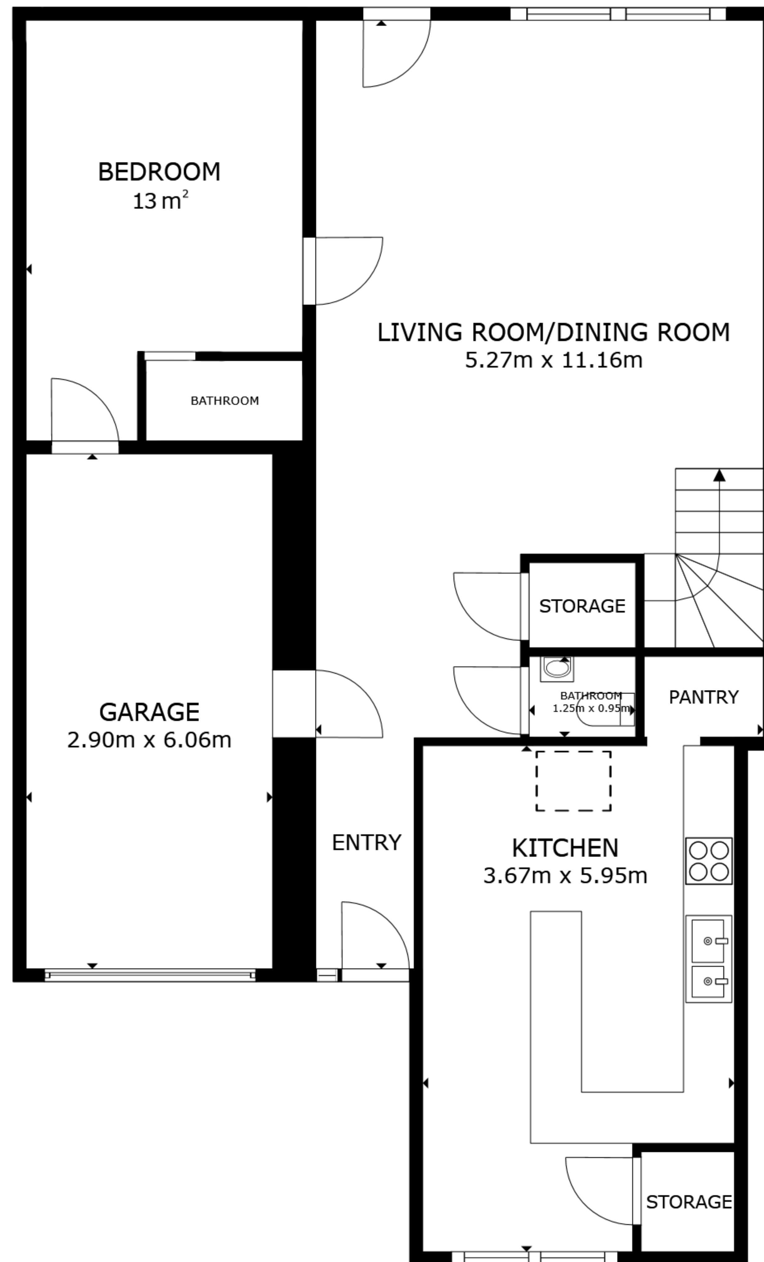
FLOOR 1
