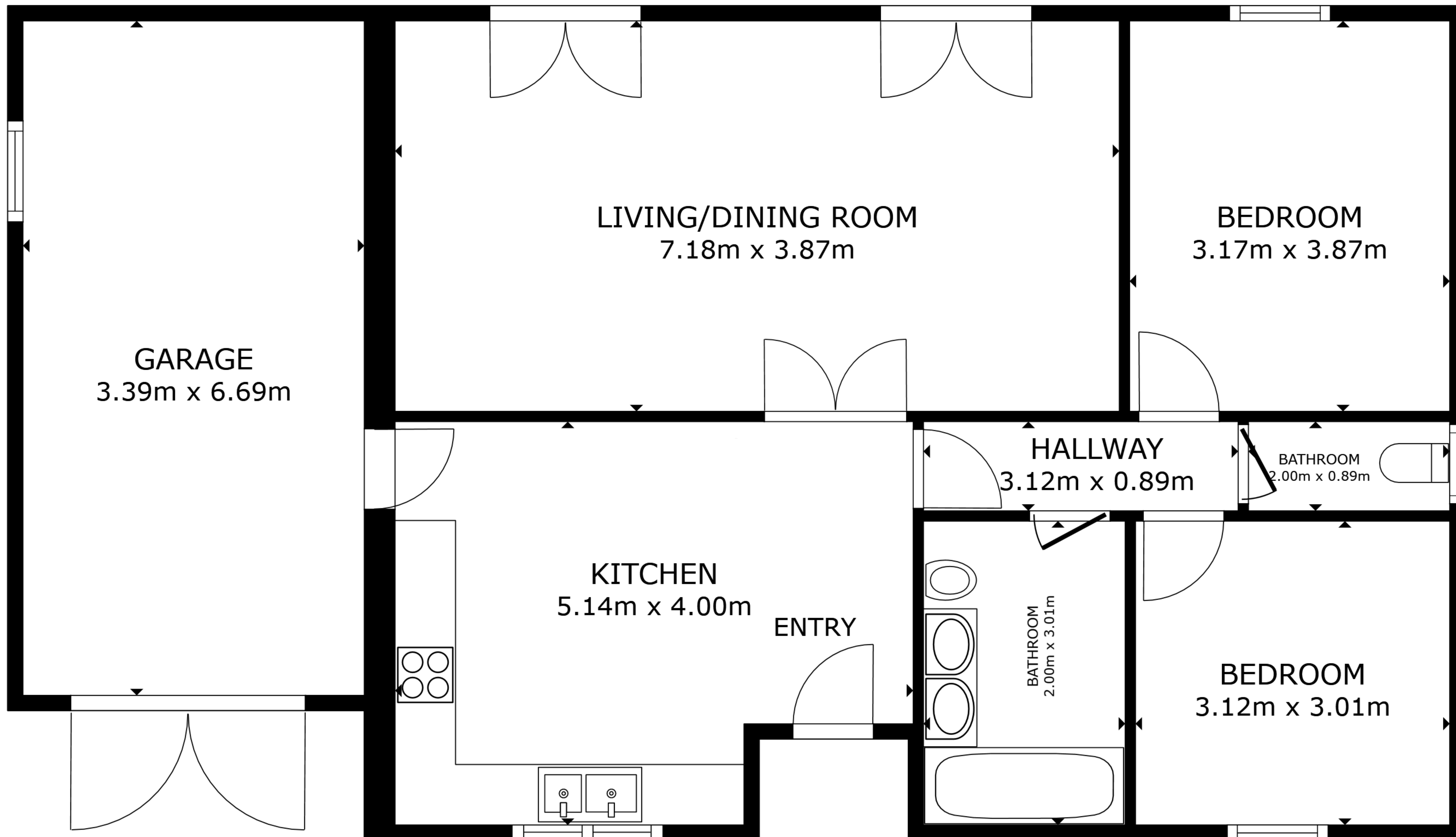
FLOOR PLAN
