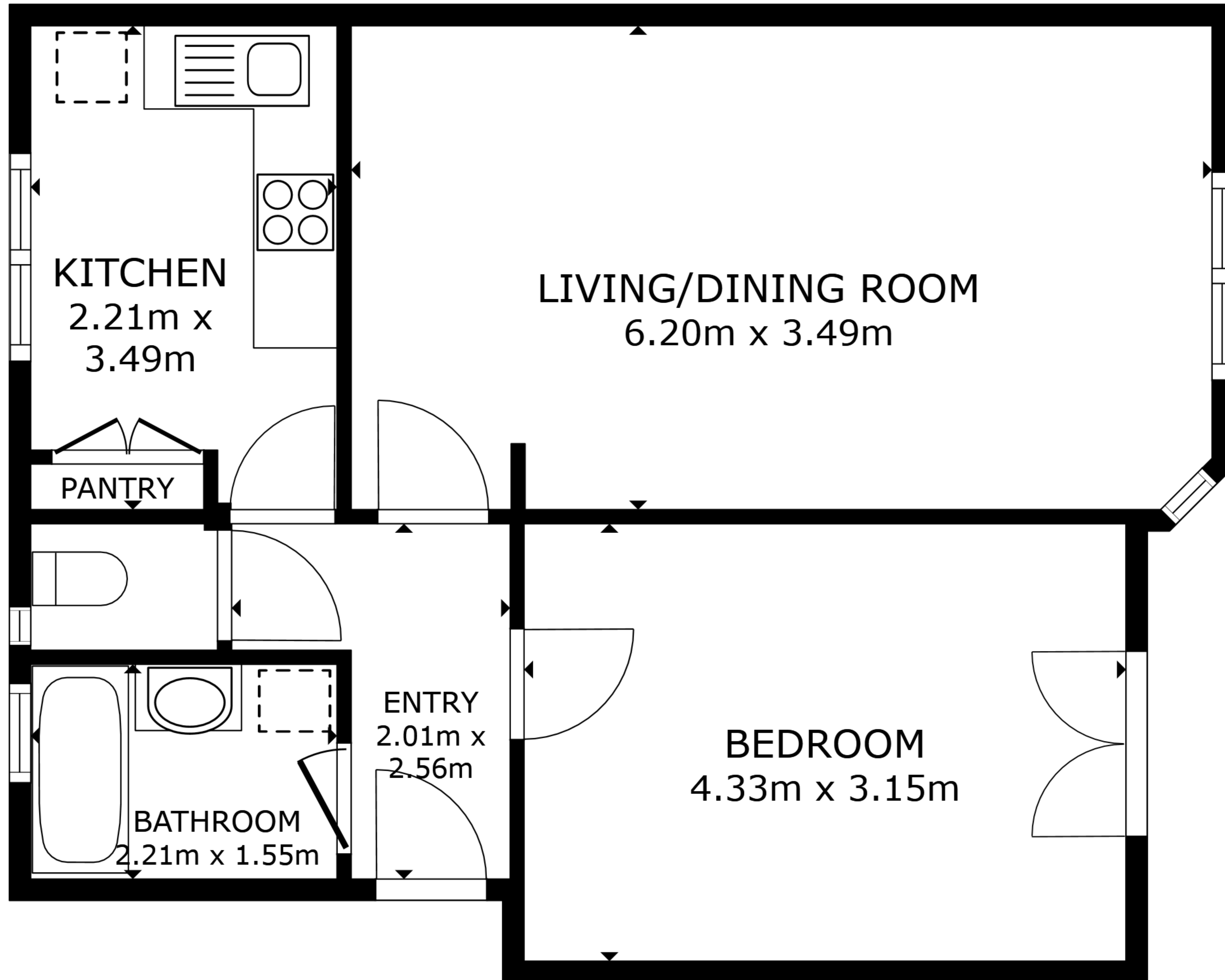
FLOOR PLAN
